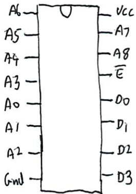
635241 512x4 PROM
